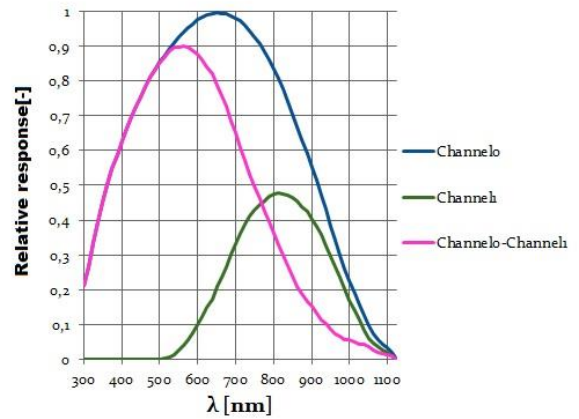
Fig.4Sensitivity of the LUX sensor[11]
