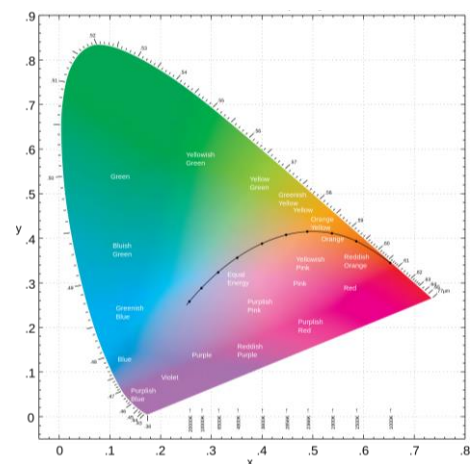
Fig.2The CIE 1931 Chromaticity Diagram [1]
