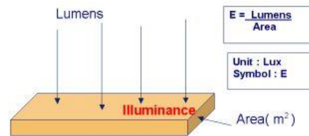
Fig.1 Illuminance definition[3]
