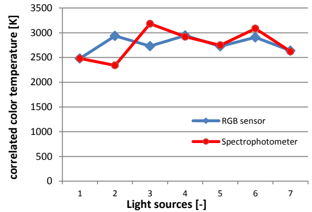
Fig.6 Measured results for CCT
