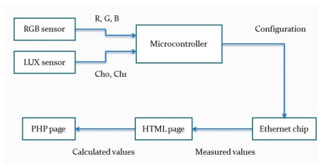
Fig.3Flow chart of the device
