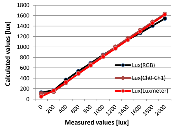
Fig.7 Measured results for illuminance
