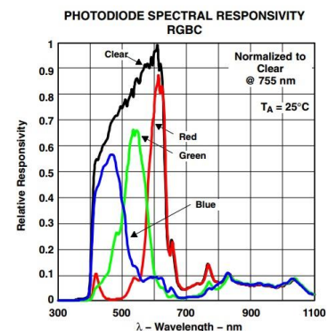
Fig.5 Sensitivity of the RGB sensor[2]
